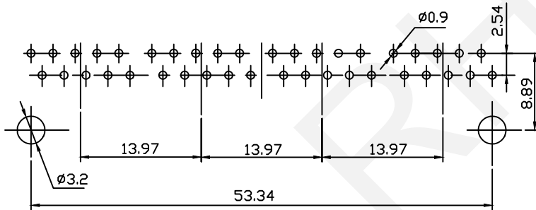
PCB Layout
